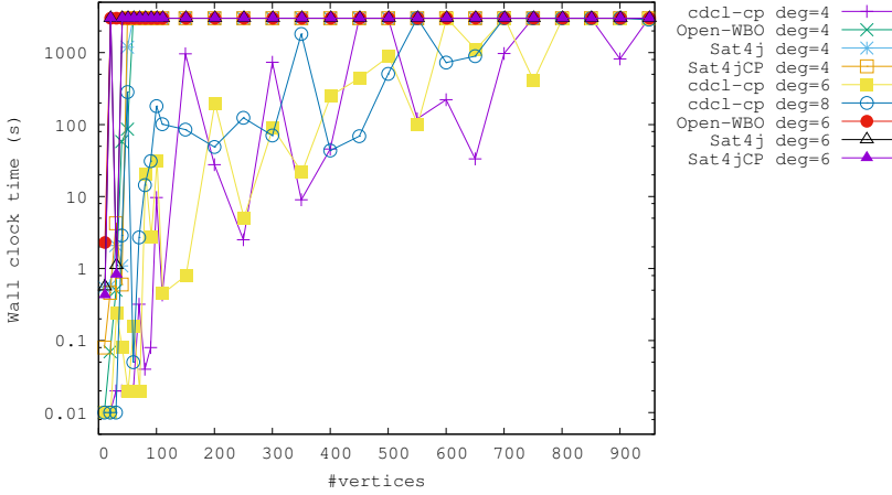
Fig. 1: Solver performance for even colouring formulas on random graphs ( \#constraints = \#vertices \ |V| ; \#variables = \deg \cdot |V|/2 + O(1) ).
