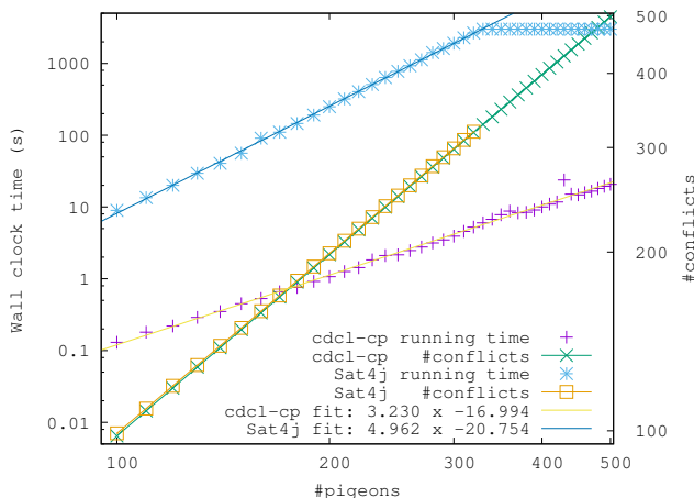
Fig. 5: Running time and #conflicts for cdcl-cuttingplanes and Sat4j on PHP ( \#variables = pigeons(pigeons - 1) , \#constraints = 2 \cdot pigeons - 1 ).
